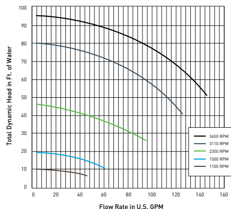
Performance Curves
